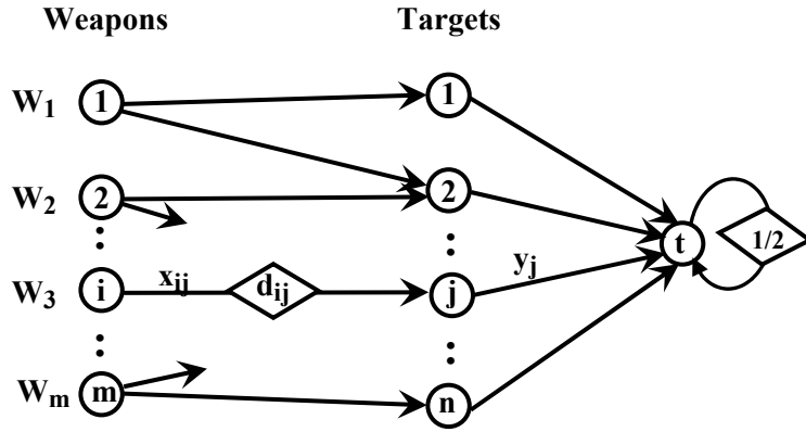
Figure 1. Formulating the WTA problem as an integer generalized network flow problem.
